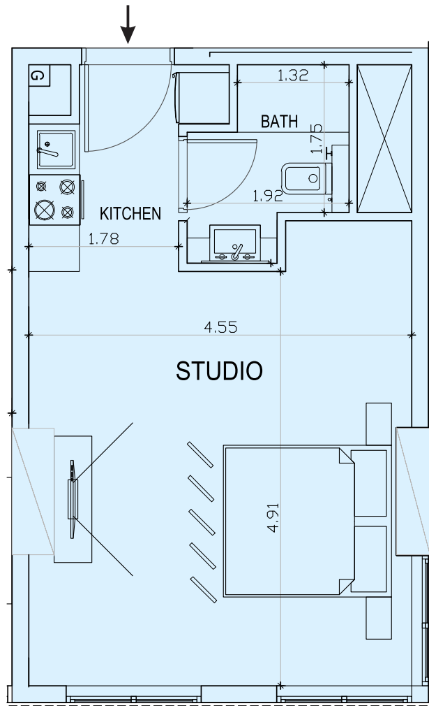
STUDIO | 03 | 02 to 06 Floors
